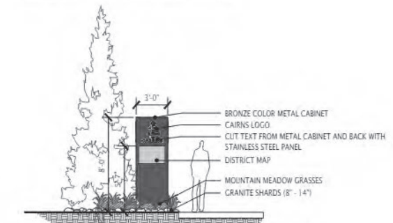
Figure 825 - Front view of a district map style pedestrian wayfinding signage
