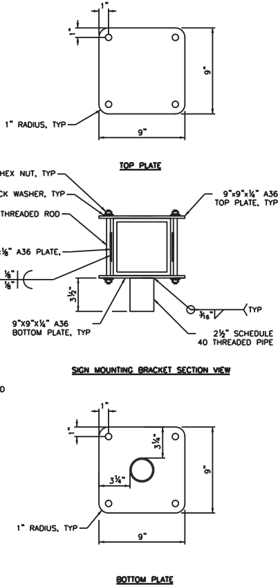
SIGN MOUNTING BRACKET
