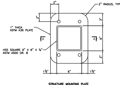
STRUCTURE MOUNTING PLATE
