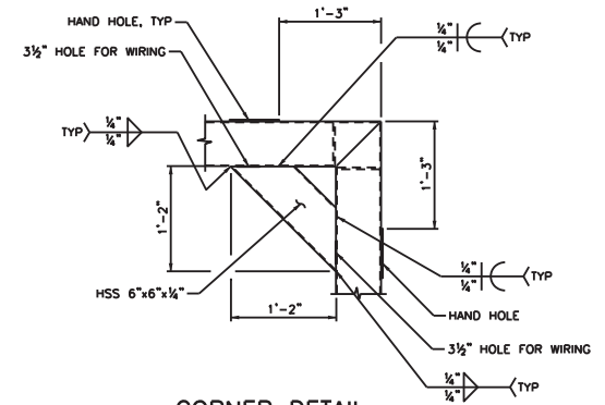
CORNER DETAIL
