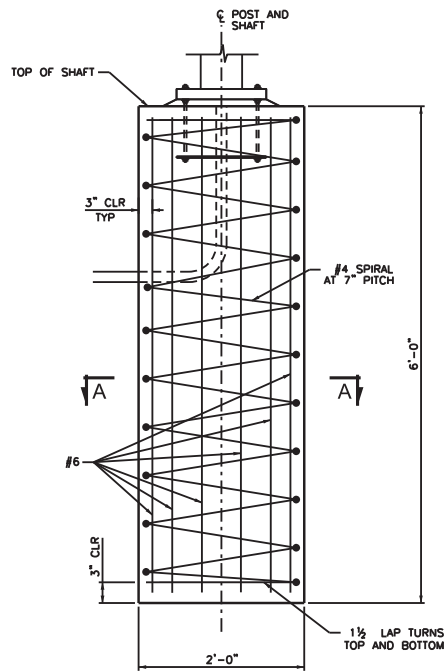
SIGN FOUNDATION
